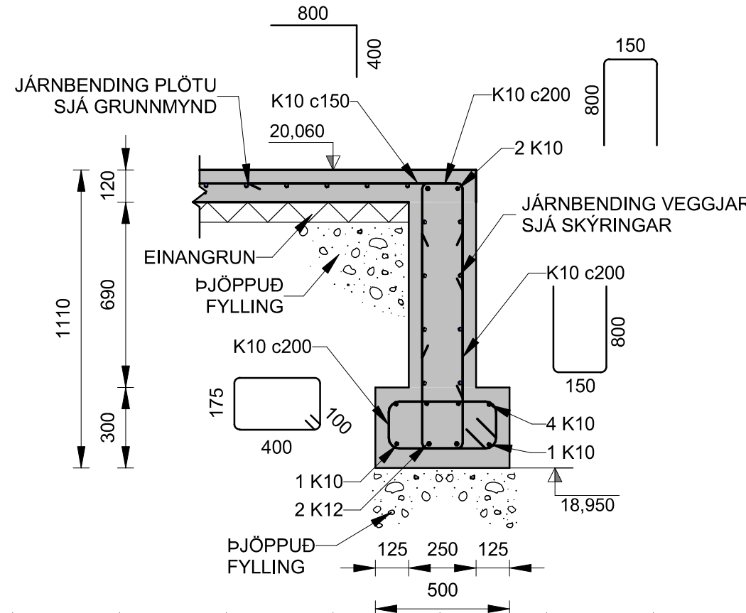
U011 SNID G001 1 : 20 G002 G003 G101 G102 G103
